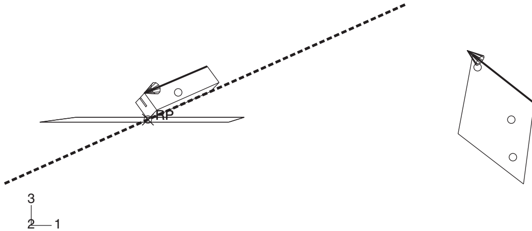
Figure 12-77 Parallel edge constraint for the circuit board.
