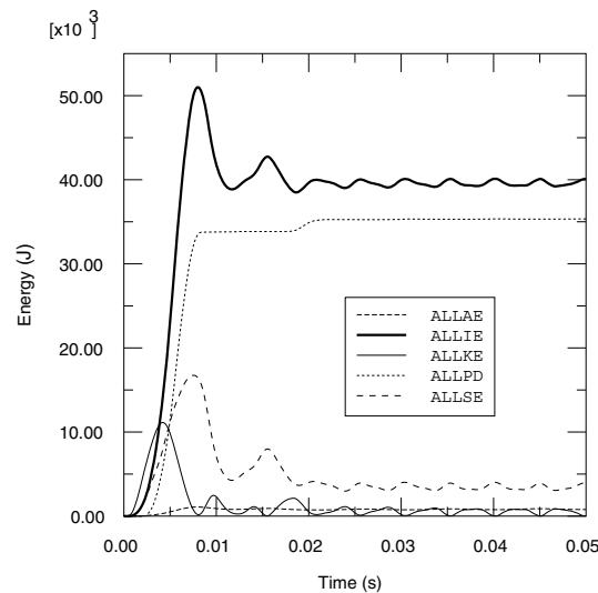
Figure 10–38 Energy quantities as a function of time.
