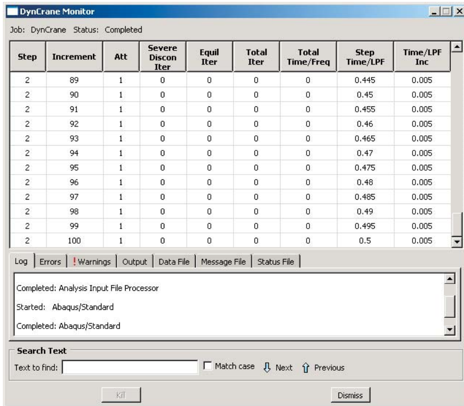
Figure 7-7 Bottom portion of the Job Monitor : cargo crane dynamic analysis.
