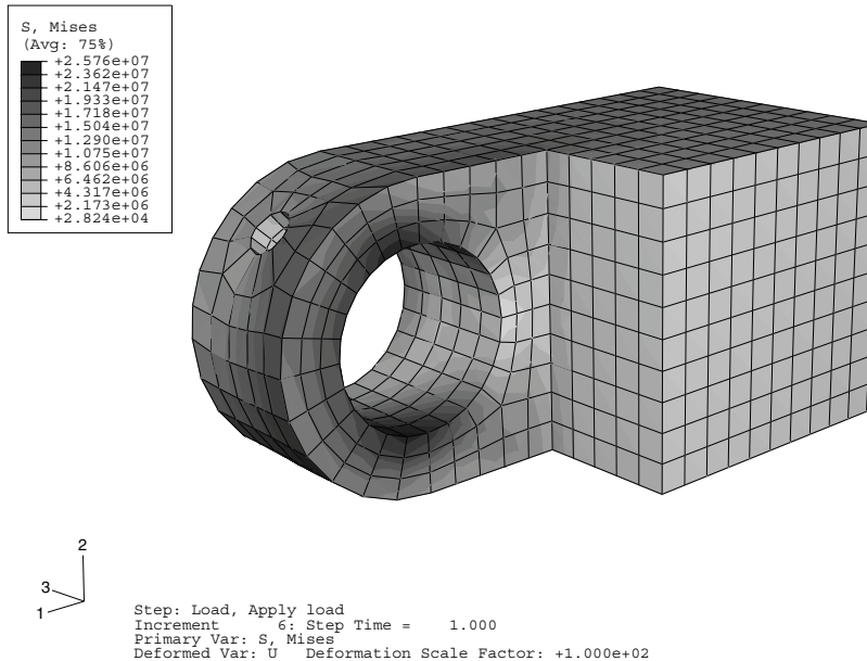
Figure C-54 Use display groups to view a contour plot of the von Mises stress in the hinge piece with the lubrication hole.
