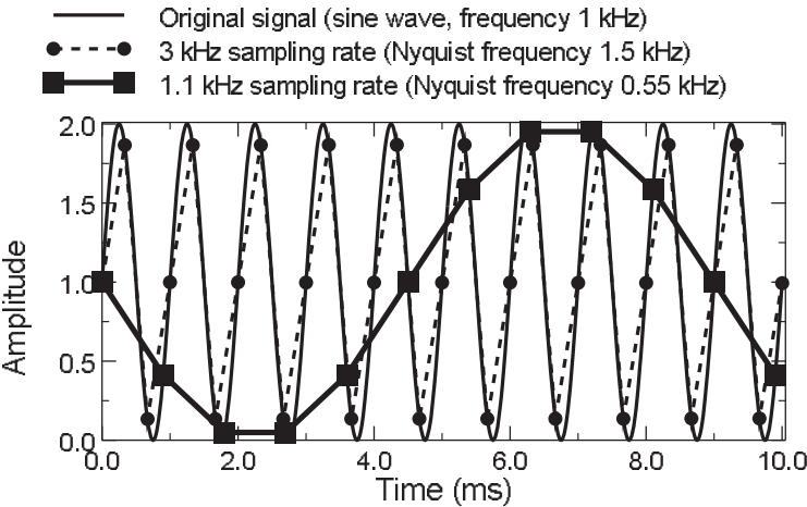
Figure 12-85 1 kHz sine wave sampled at 1.1 kHz and 3 kHz.
