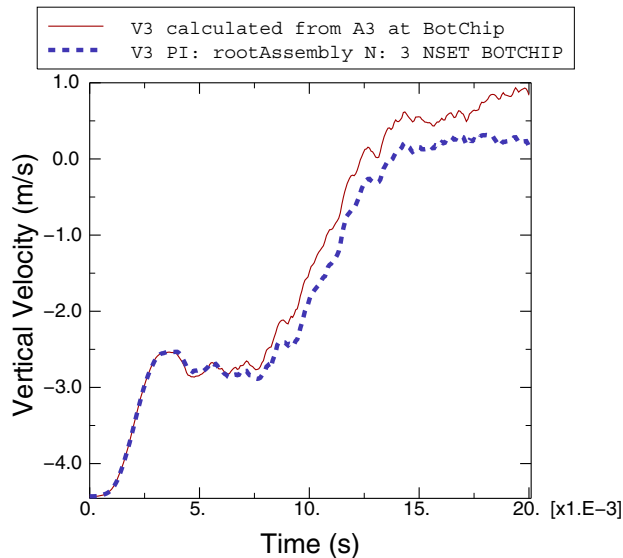
Figure 12–83 Velocity of the bottom chip in the Z-direction.
