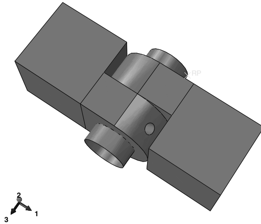
Figure C–35 Shaded view of the finished assembly.
