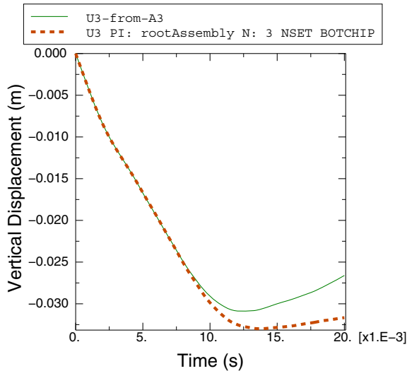
Figure 12-84 Displacement of the bottom chip in the Z-direction.
