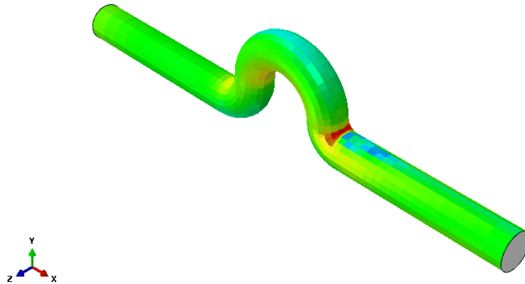
Figure E–18 YPLUS contour plot.
