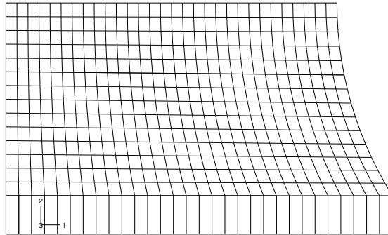
Figure 10-63 Undeformed model shape of the rubber mount.
