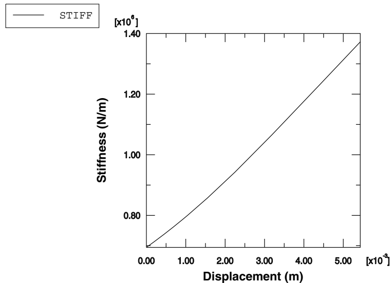
Figure 10–62 Stiffness characteristic of the mount.
