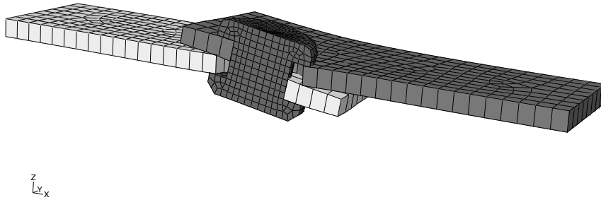
Figure 12–48 Deformed model shape.
