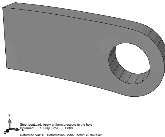
Figure 4–27 Deformed shape with only feature edges visible.
