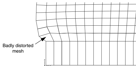
Figure 10–65 Distortion at the left-hand corner of the rubber mount model.
