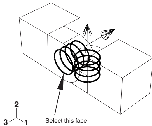
Figure C-28 Select a cylindrical face on the fixed instance.
