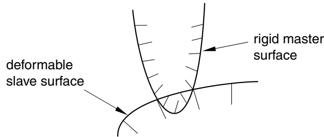
Figure 12-62 Example of inadequate slave surface discretization.
