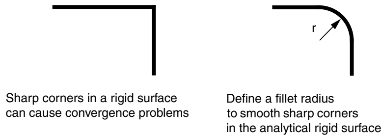
Figure 12-12 Smoothing an analytical rigid surface.
