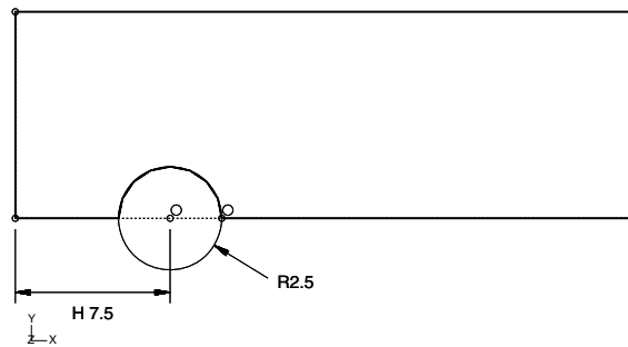
Figure 12-33 Sketch of the bolt hole.
