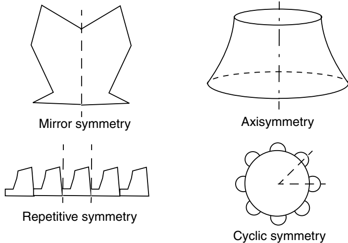
Figure 10-49 Various forms of symmetry.
