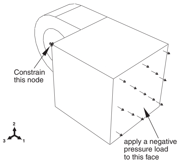
Figure C-42 The second hinge is constrained and loaded.
