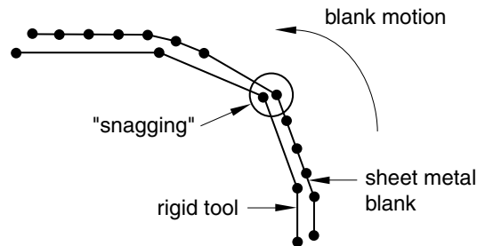
Figure 12–61 Potential effect of coarse rigid body discretization.
