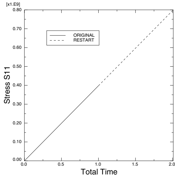
Figure 11–12 History of axial stress in the pipe.
