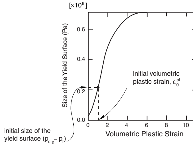
Figure 12-70 Foam hardening material data.
