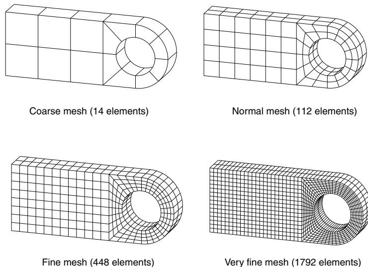
Figure 4–44 Different meshes for the connecting lug problem.
