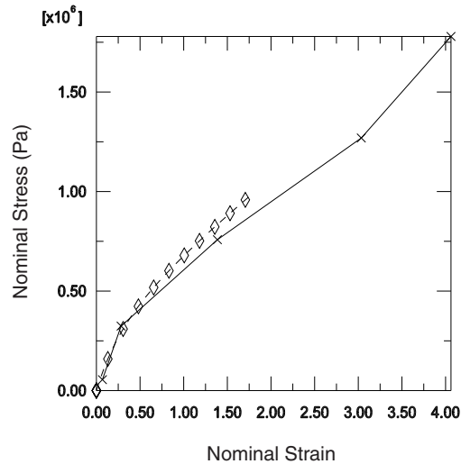
Figure 10-56 Comparison of experimental data (solid line) and Abaqus/Standard results (dashed line): planar shear.
