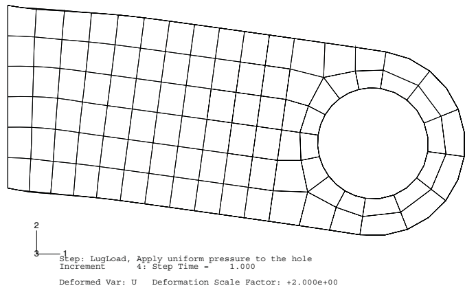
Figure 10–19 Deformed model shape for the simulation with plastic hardening.
