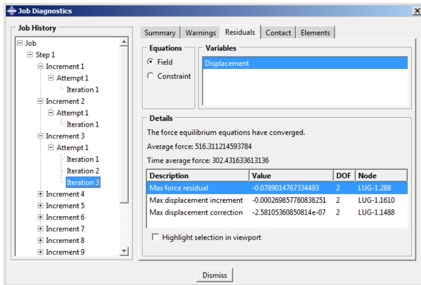
Figure 10–14 Convergence history for Increment 3 .
