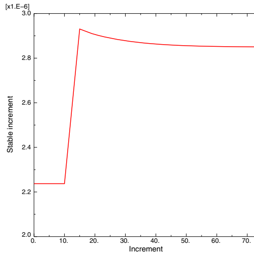
Figure 9-8 Stable time increment history.
