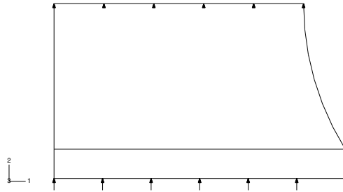
Figure 10–60 Boundary conditions on the rubber mount; pressure loading on the steel plate.
