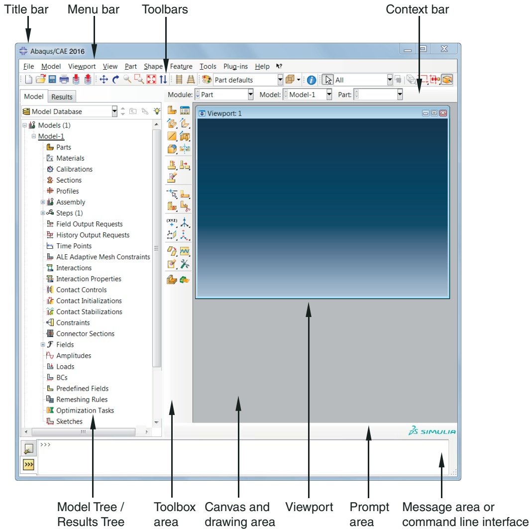
Figure 2–2 Components of the main window.
