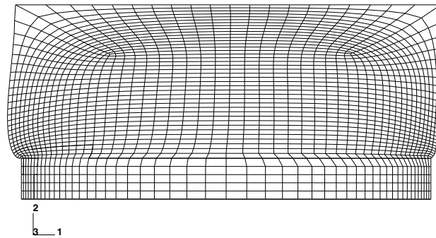
Figure 10-71 Deformed shape of the modified mesh.
