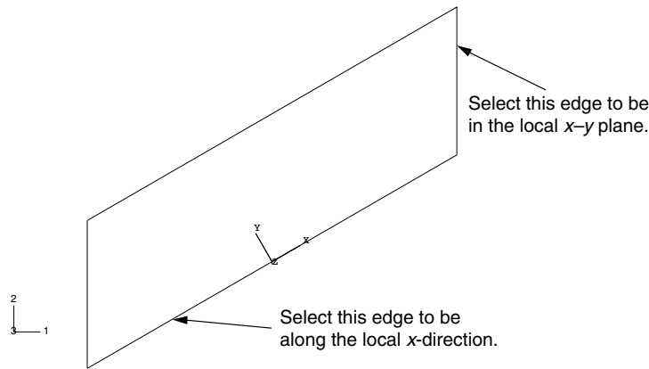
Figure 5–11 Datum coordinate system used to define local material directions.
