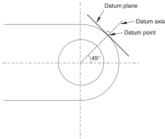
Figure C–11 Two-dimensional view of the datum plane's position with respect to the hinge piece.
