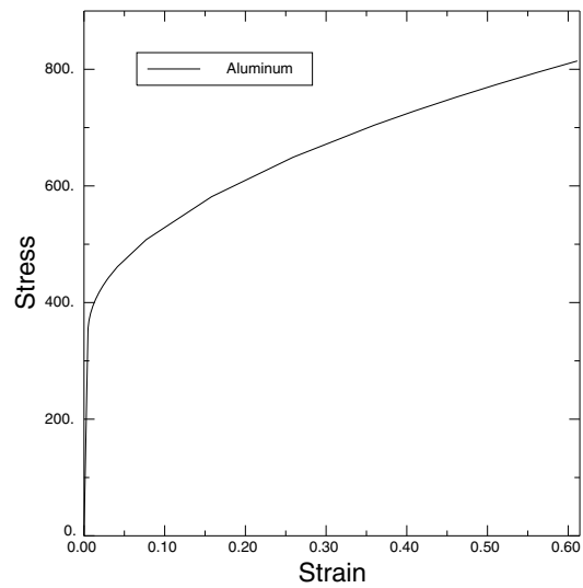
Figure 12-37 Aluminum stress-strain curve.
