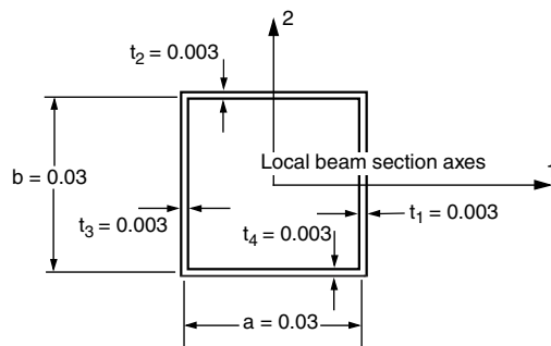
Figure 6–20 Cross-section geometry and dimensions (in m) of the internal and cross bracing members.
