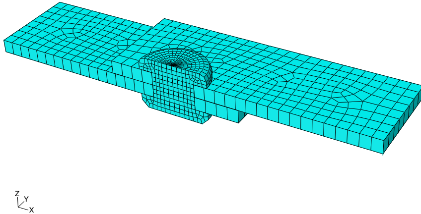
Figure 12–47 Meshed assembly.
