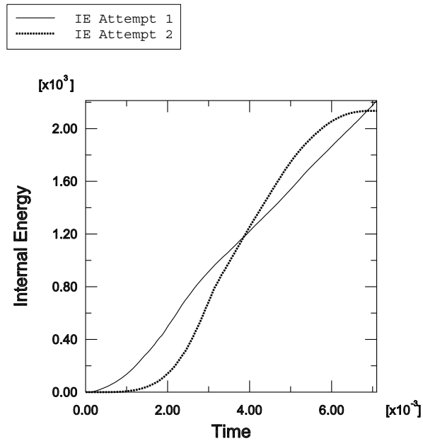
Figure 13-12 Internal energy history for forming analysis, attempt 2.
