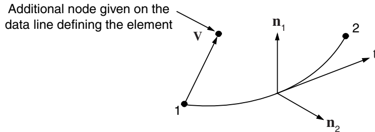
Figure 6–3 Orientation of the beam element tangent, \mathbf{t} , and beam section axes, \mathbf{n}_1 and \mathbf{n}_2 .
