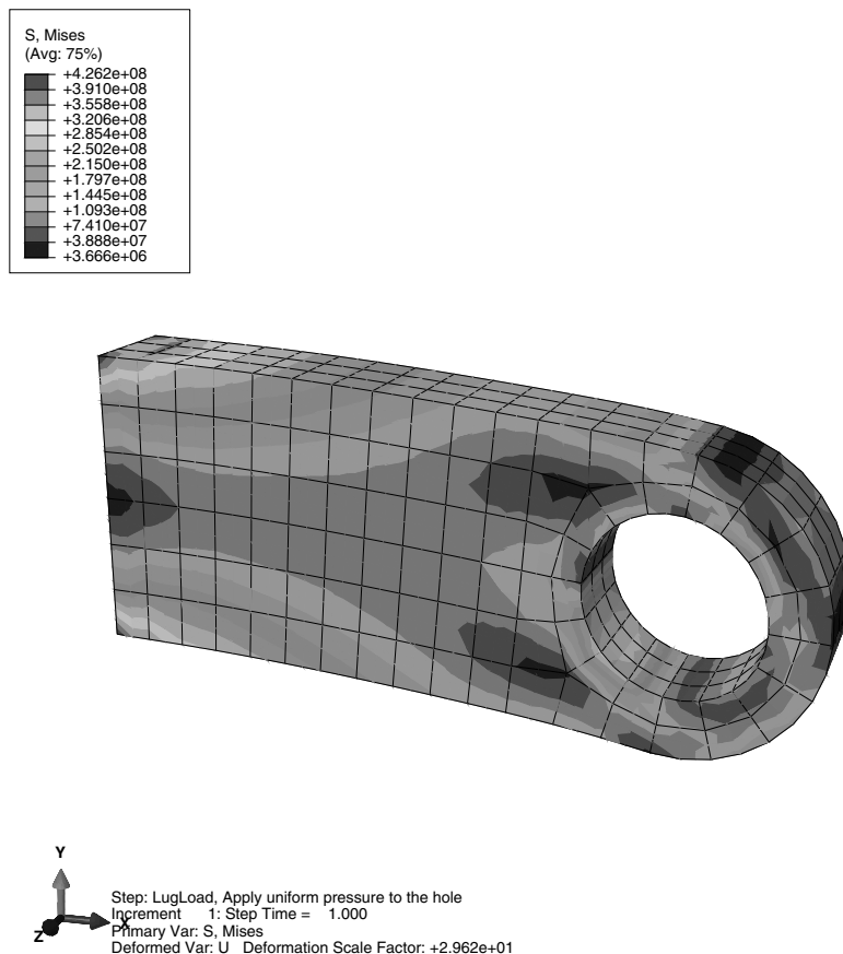
Figure 4–31 Filled contour plot of Mises stress.
