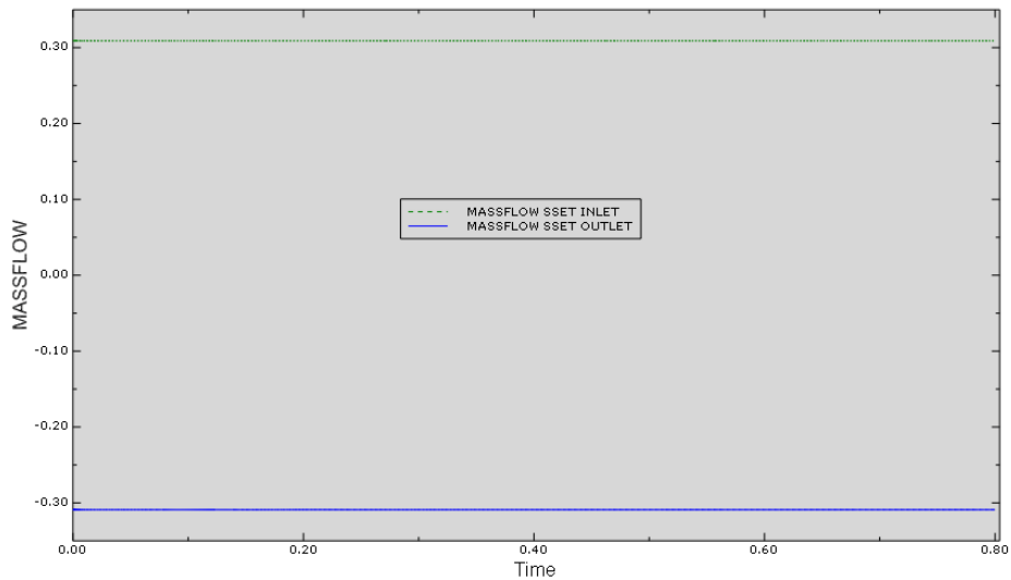
Figure E–19 Mass flow rates at inlet and outlet.
