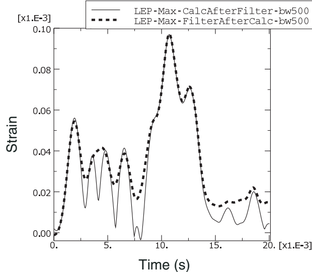
Figure 12–91 Principal logarithmic strain calculated before and after filtering (cutoff frequency 500 Hz).
