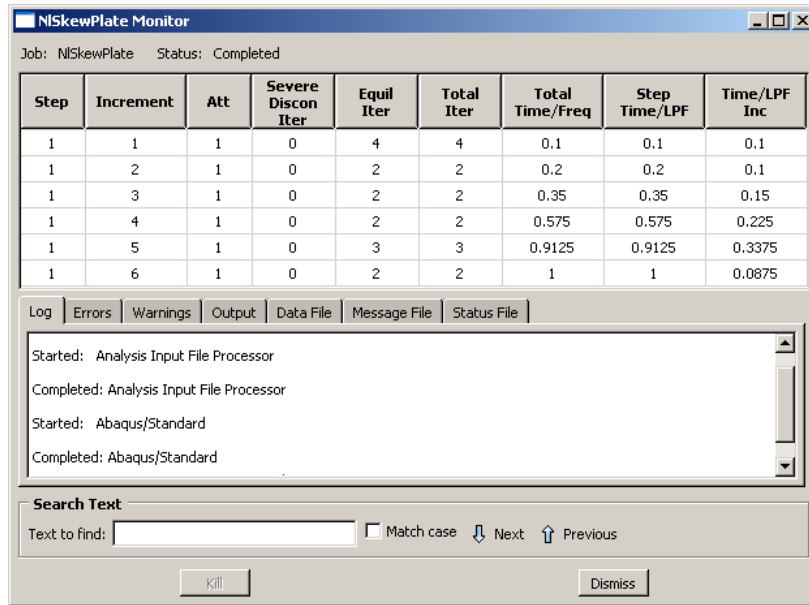
Figure 8–12 Job Monitor: nonlinear skew plate analysis.
