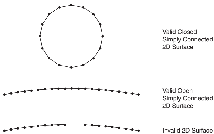
Figure 12-54 Valid and invalid two-dimensional surfaces for the contact pair algorithm.
