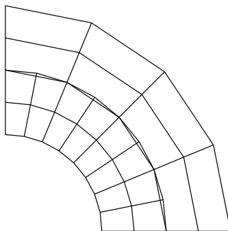
Figure 12-63 Original overclosure of two contact surfaces.
