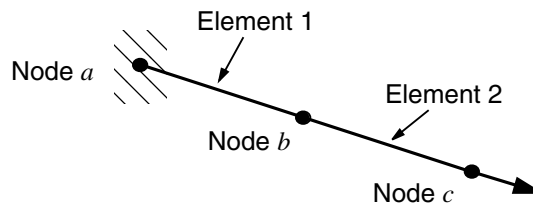
Figure 1-5 Discretized model of the truss problem.
