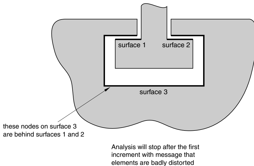
Figure 12–59 Example of an incorrect surface definition.
