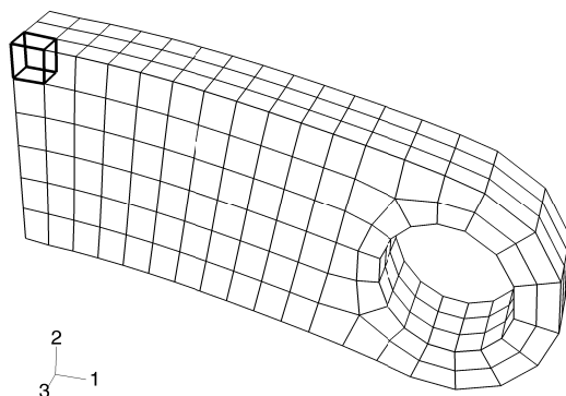
Figure 4–42 Selected element near the built-in end of the lug.
