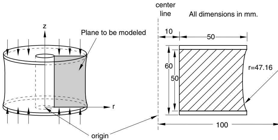
Figure 10–48 Axisymmetric mount.
