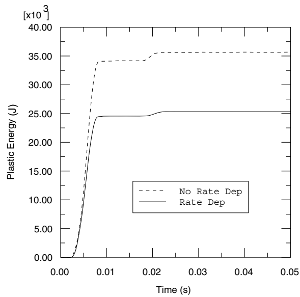
Figure 10-45 Plastic strain energy with and without rate dependence.
