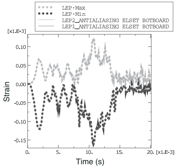
Figure 12–90 Principal logarithmic strain values versus time.
