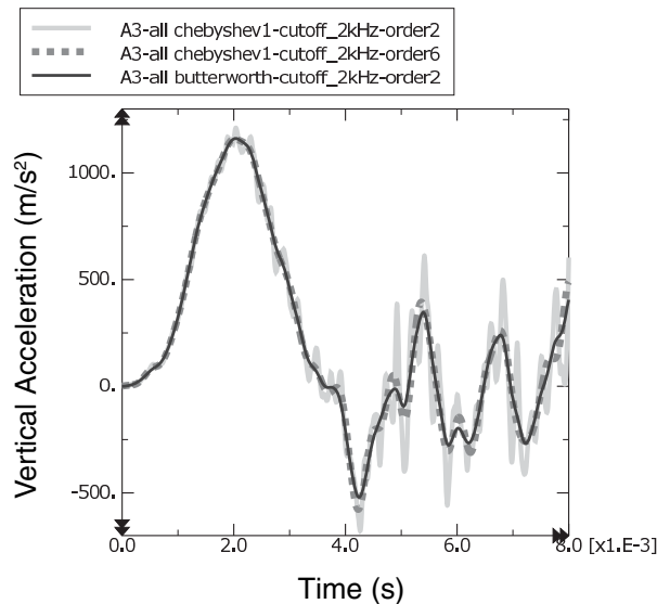
Figure 12-89 Comparison of acceleration filtered with Butterworth and Chebyshev Type I filters.
