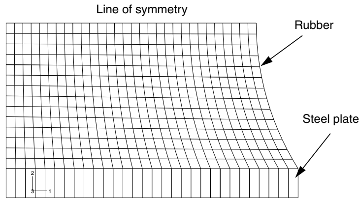
Figure 10-61 Mesh for the rubber mount.
