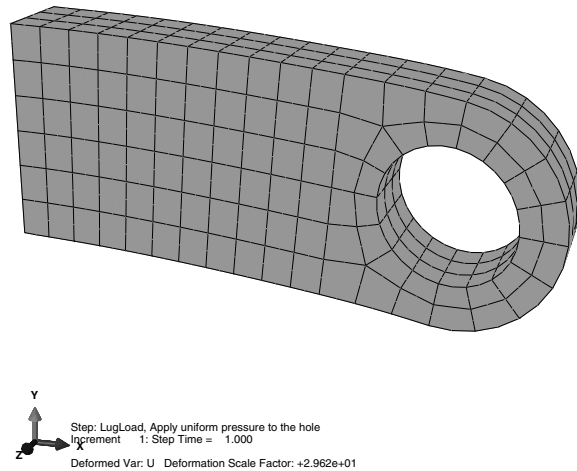
Figure 4–30 Filled element plot.
