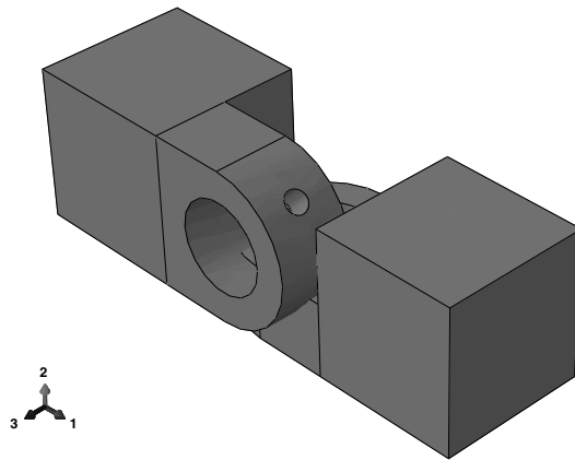
Figure C–26 Position 1: Constrain the flange of the solid hinge piece to face the flange of the hinge piece with the lubrication hole.
