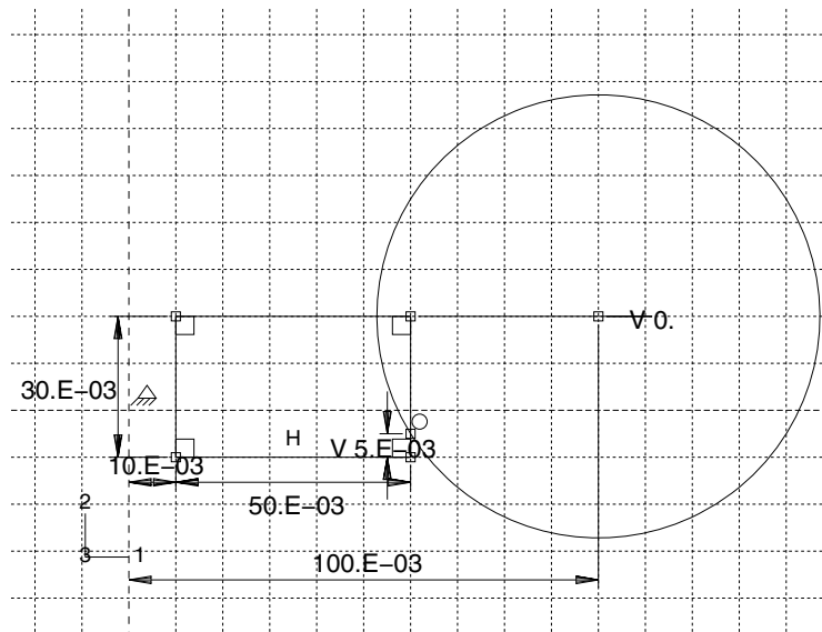
Figure 10-51 Construction geometry used to create the part (with grid spacing doubled).
