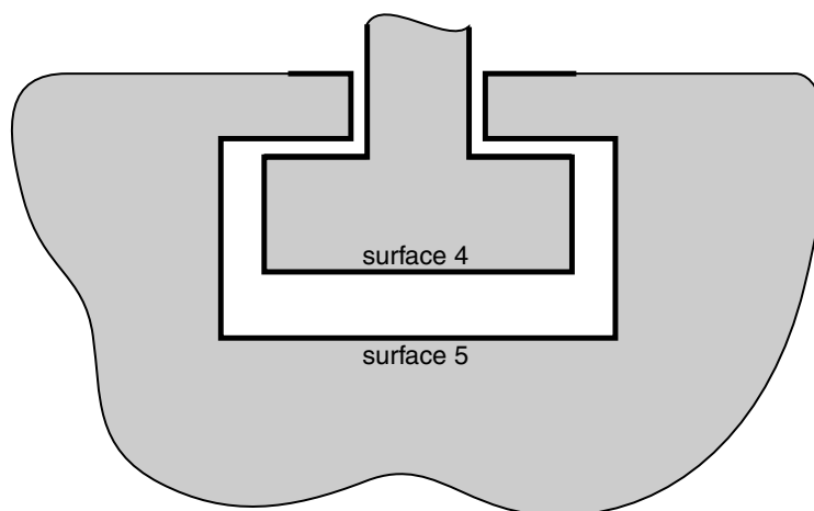
Figure 12–60 Correct surface definition.
