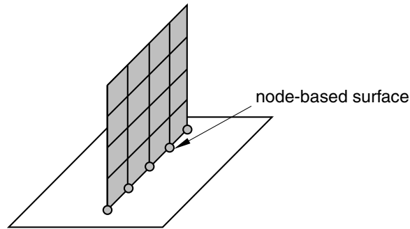
Figure 12-2 Node-based region for contact on a shell edge.
