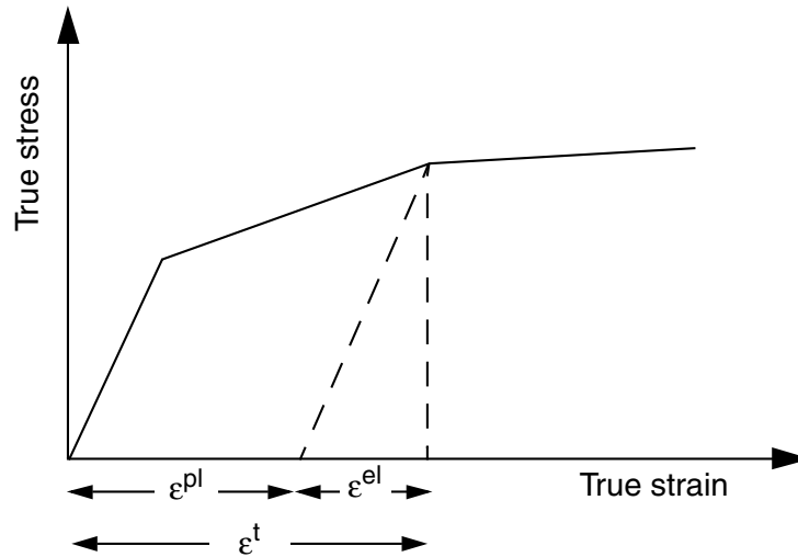
Figure 10–3 Decomposition of the total strain into elastic and plastic components.
