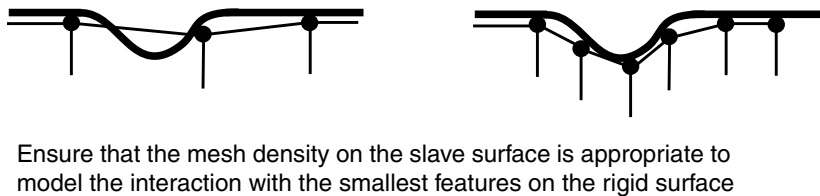
Figure 12–11 Modeling small features on the rigid surface.
