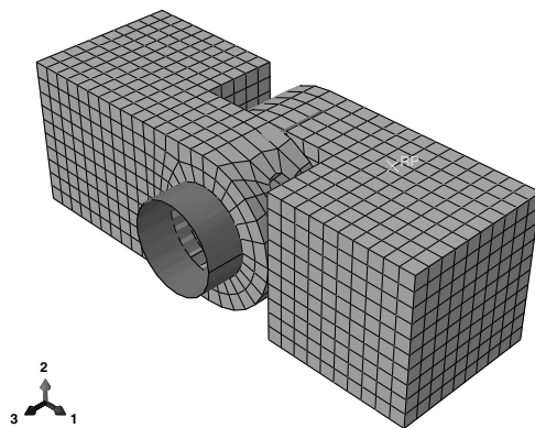
Figure C-52 Final view of the meshed model.
