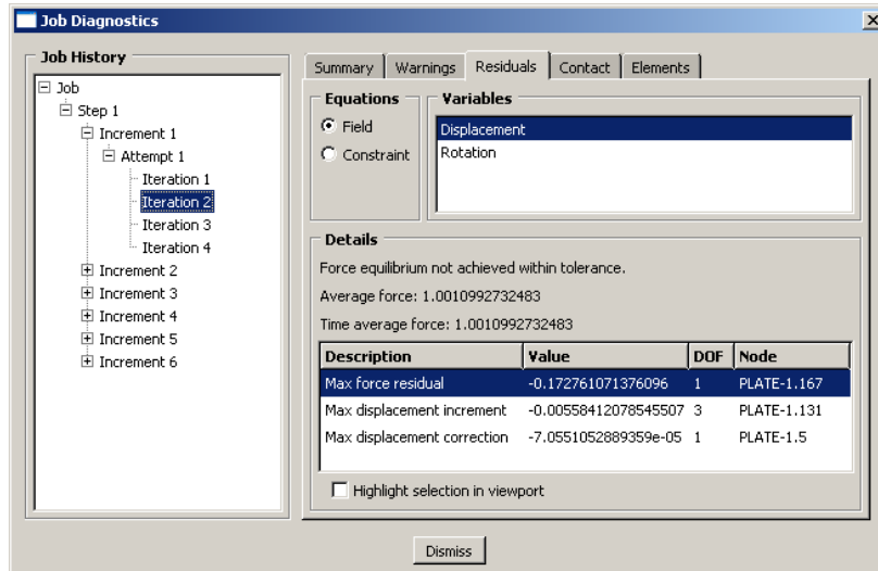
Figure 8–15 Force residual information for the second iteration.
