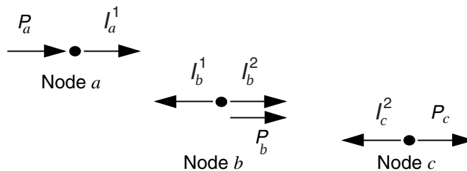
Figure 1-6 Free-body diagram for each node.
