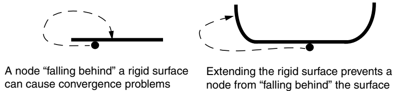
Figure 12–10 Extending rigid surfaces to prevent convergence problems.
