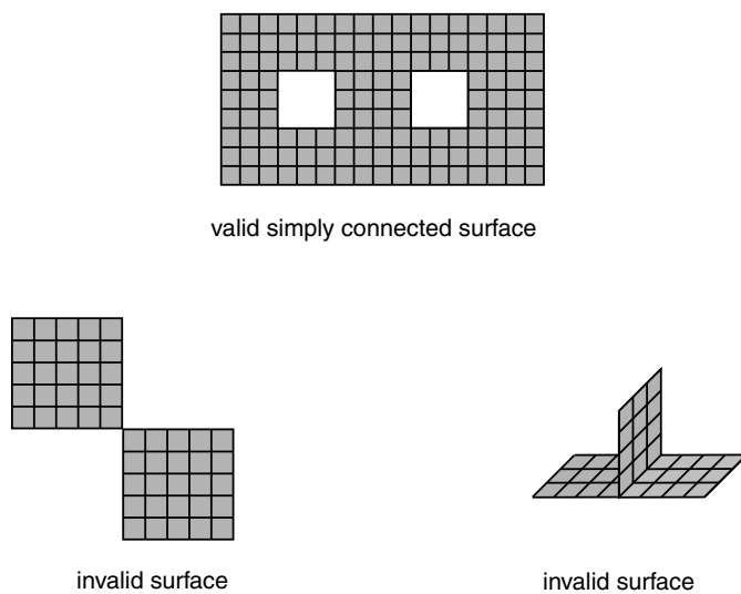
Figure 12-55 Valid and invalid three-dimensional surfaces for the contact pair algorithm.
