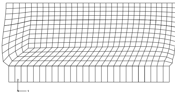
Figure 10-68 Deformed shape of the modified mesh.
