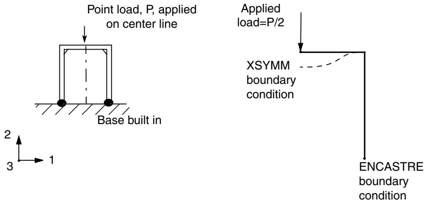
Figure 10-50 Symmetric portal frame.
