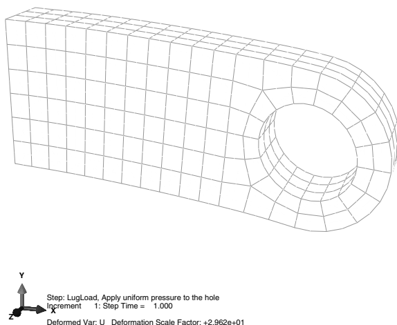
Figure 4–29 Hidden line plot.
