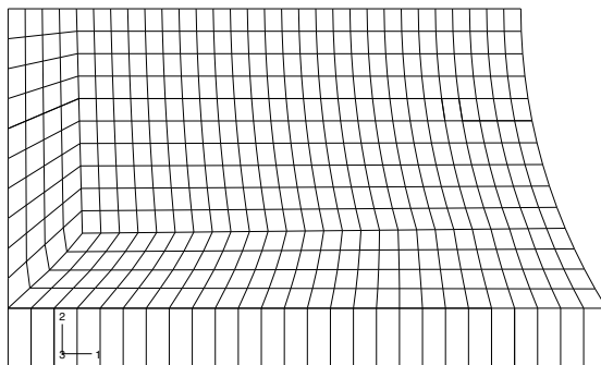
Figure 10-67 Modified mesh to minimize element distortions in the bottom left corner of the rubber model during the simulation.
