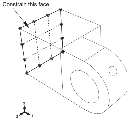
Figure C-40 One end of the hinge is constrained.
