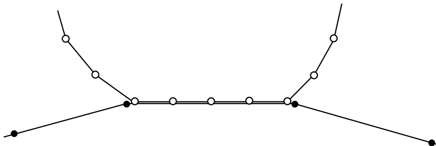
Figure 12-53 Balanced master-slave contact constraint with kinematic compliance.
