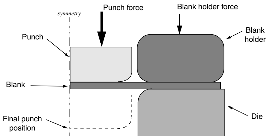
Figure 12–14 Forming analysis.
