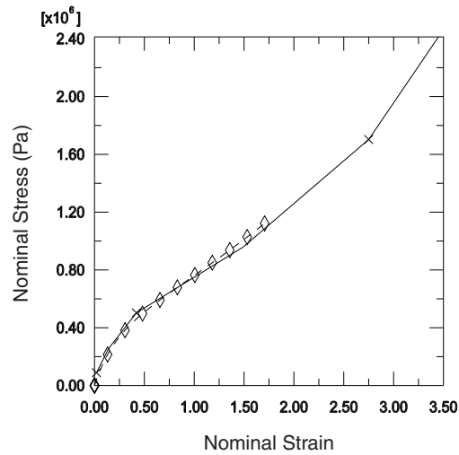
Figure 10-54 Comparison of experimental data (solid line) and Abaqus/Standard results (dashed line): biaxial tension.
