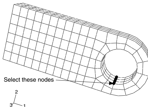
Figure 4–36 Nodes in display group nodes at hole bottom .
