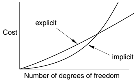
Figure 2–20 Cost versus model size in using the explicit and implicit methods.
