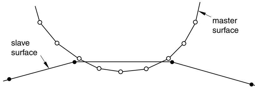
Figure 12-52 Penetration of master nodes into slave surface with pure master-slave contact.
