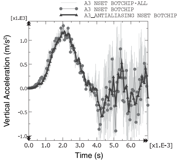
Figure 12–86 Comparison of acceleration output with and without filtering.
