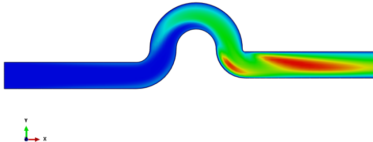
Figure E-17 Turbulent viscosity contour plot.
