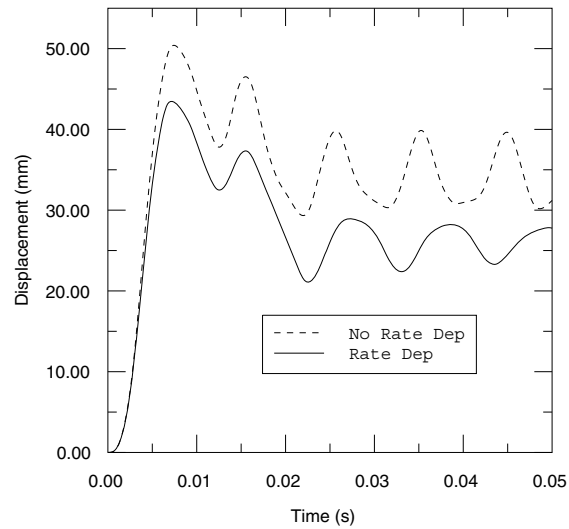
Figure 10-44 Displacement of the central node with and without rate dependence.
