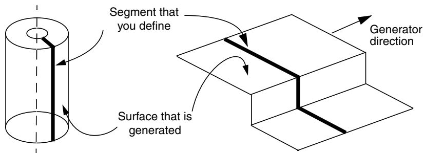
Figure 12-3 Analytical rigid surfaces.
