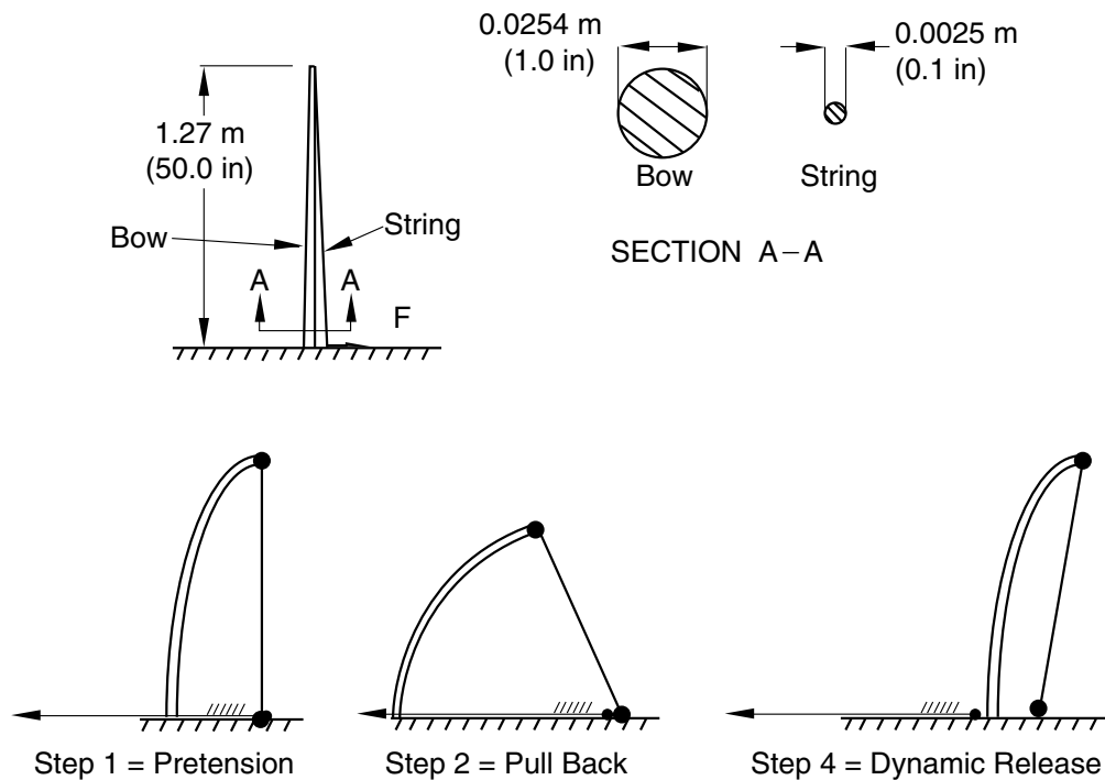
Figure 11–3 Simple bow and arrow.
