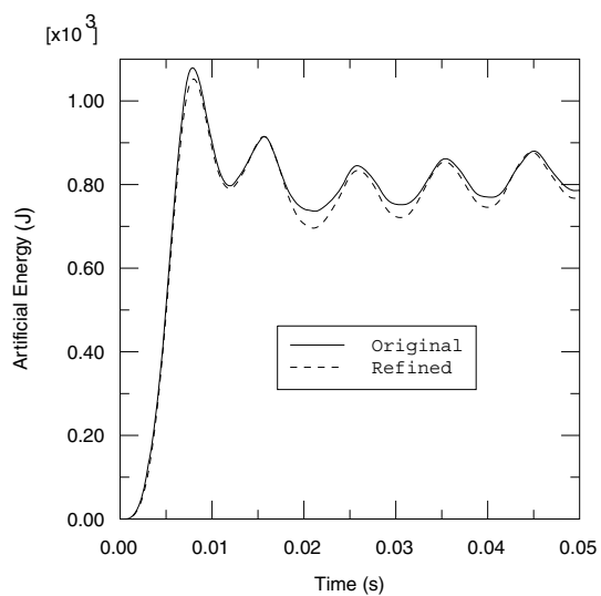
Figure 10-39 Artificial energy in the original and refined meshes.
