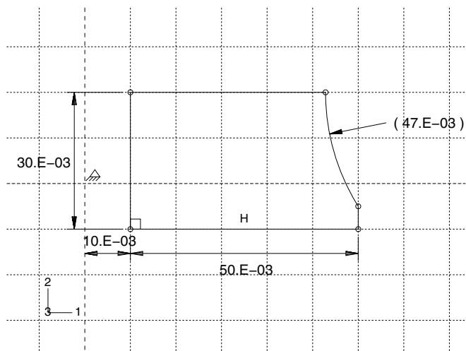
Figure 10-52 Final part geometry (with grid spacing doubled).
