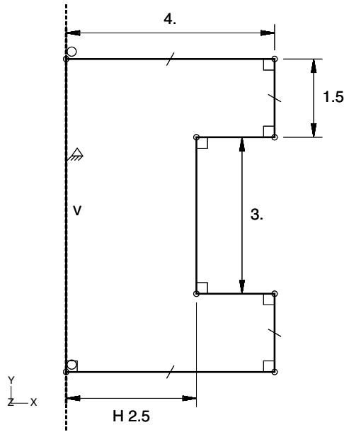
Figure 12–35 Base sketch of the rivet.
