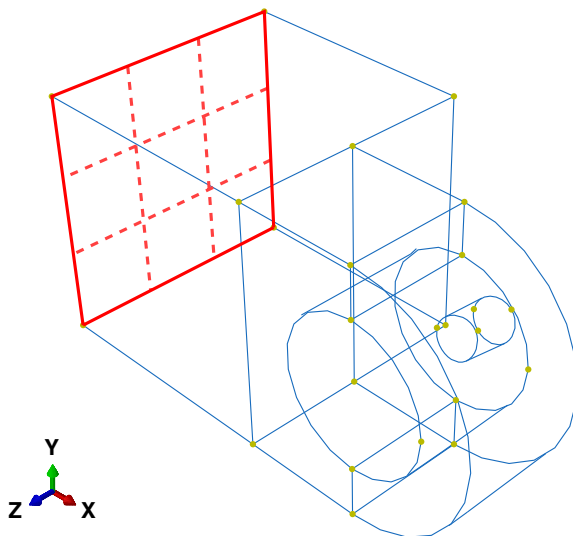
Figure C–43 Apply a boundary condition to the end of the hinge piece with the lubrication hole.
