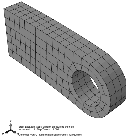
Figure 4–25 Deformed model shape of connecting lug (shaded).
