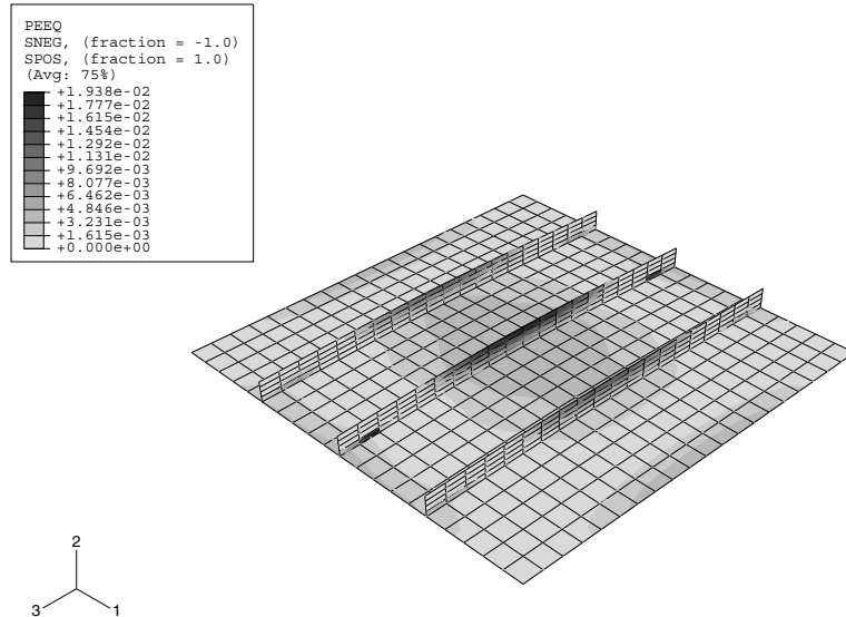
Figure 10–42 Contour plot of equivalent plastic strain at 50 ms.
