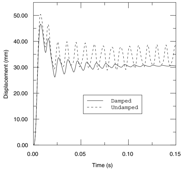
Figure 10-43 Damped and undamped displacement histories.
