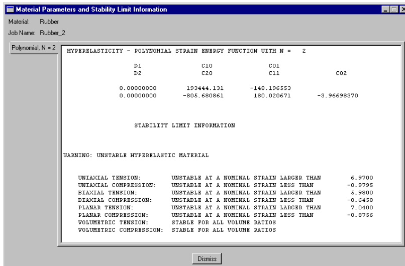
Figure 10-58 Material parameters and stability limits for the second-order polynomial strain energy function.
