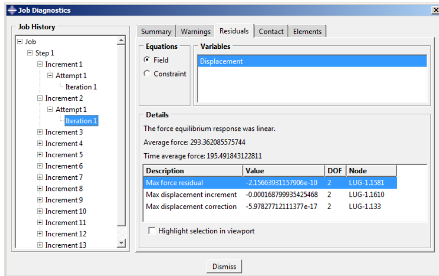
Figure 10–13 Convergence history for Increment 2 .
