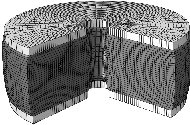
Figure 10–64 Deformed model shape of the rubber under an applied load of 5500 N (mirrored/swept image).
