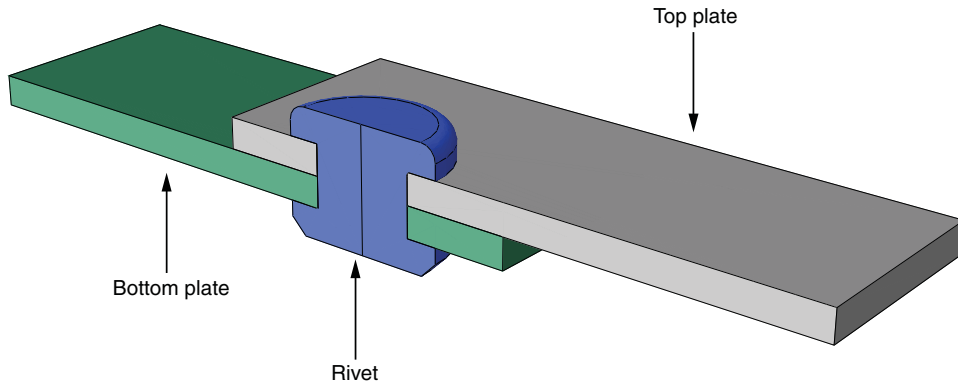
Figure 12–31 Lap joint analysis.
