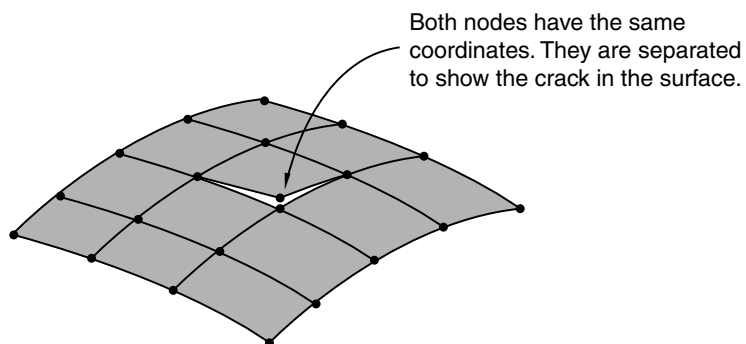
Figure 12-58 Example of a double-noded mesh.
