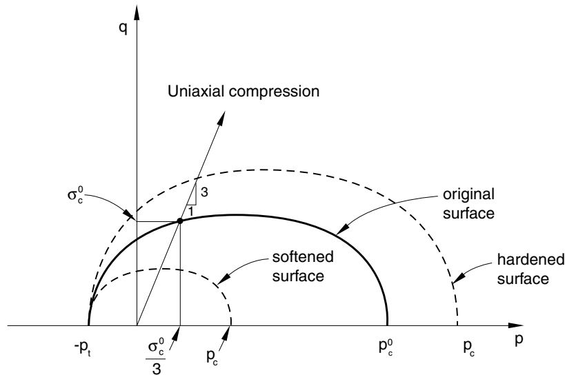
Figure 12-69 Crushable foam model: yield surface in the p - q plane.
