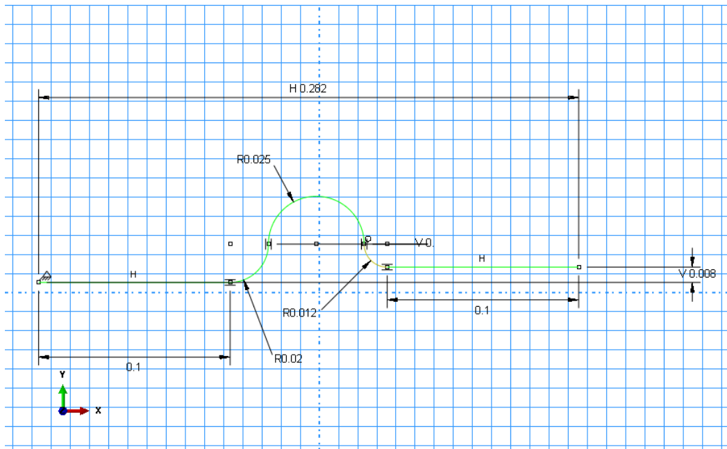
Figure E-2 Sweep path for the fluid part.
