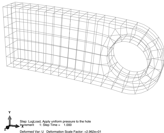
Figure 4–28 Wireframe plot.
