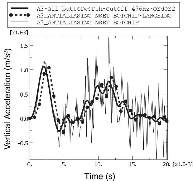
Figure 12-88 Comparison of acceleration filtered in Abaqus/Explicit and the Visualization module.
