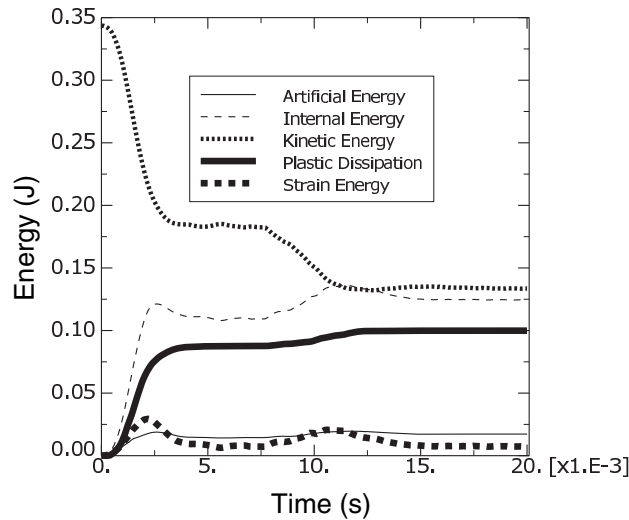
Figure 12–81 Energy results versus time.
