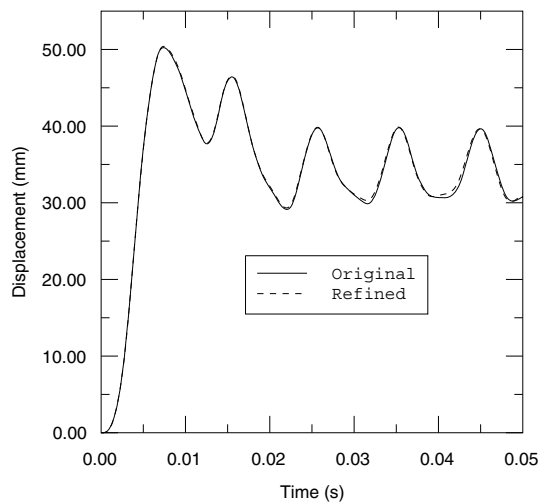
Figure 10-40 Central node displacement history for the original and refined meshes.
