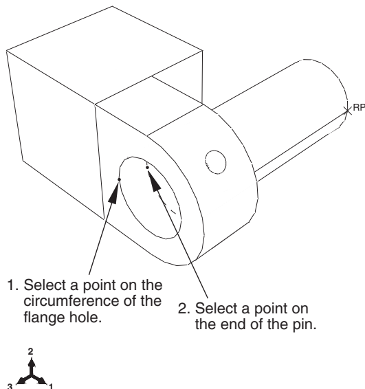
Figure C–34 Determining the position of the pin.
