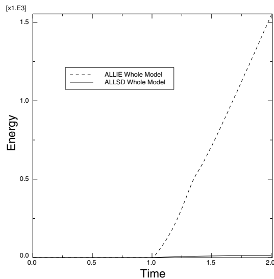
Figure 12–28 Stabilization and internal energies.
