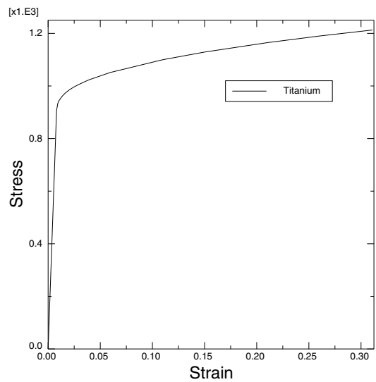
Figure 12-38 Titanium stress-strain curve.
