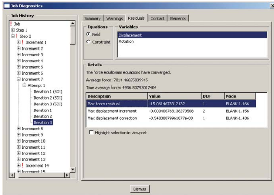
Figure 12–24 Converged equilibrium iteration.
