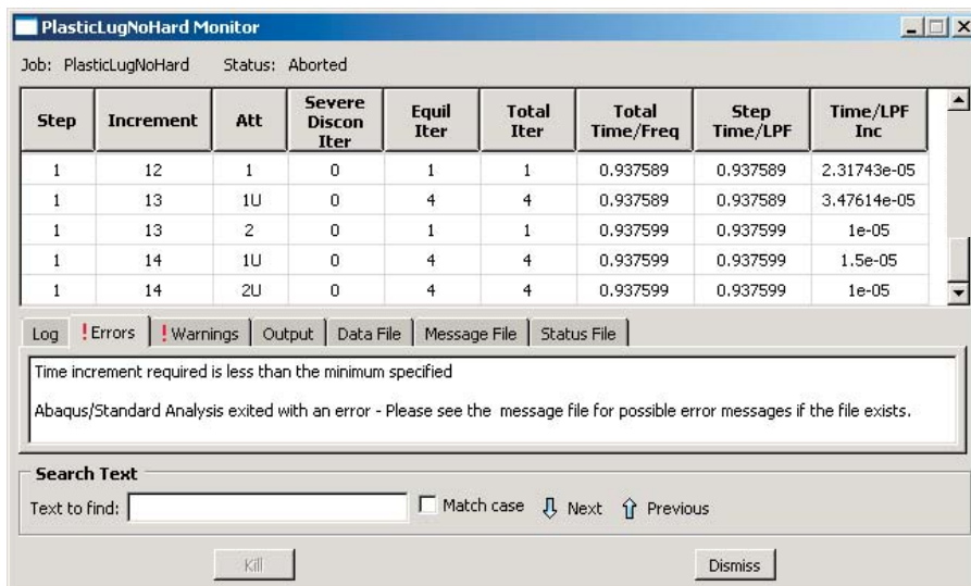
Figure 10–9 Job Monitor: perfectly plastic connecting lug.
