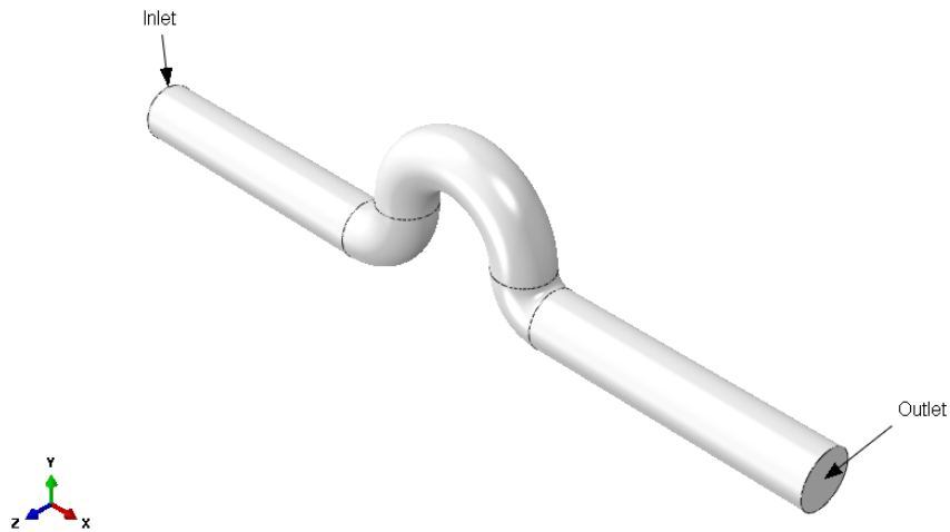
Figure E-4 Fluid part.
