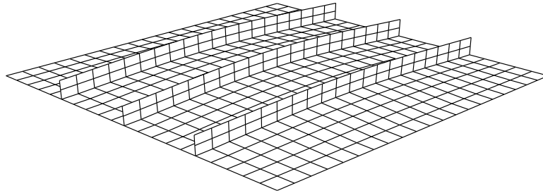
Figure 10–36 Displaced shape at 8 ms.
