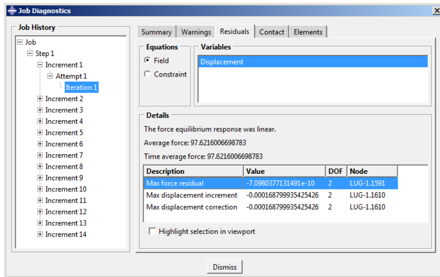
Figure 10–12 Convergence history for Increment 1 .
