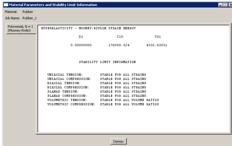
Figure 10-57 Material parameters and stability limits for the first-order polynomial strain energy function.
