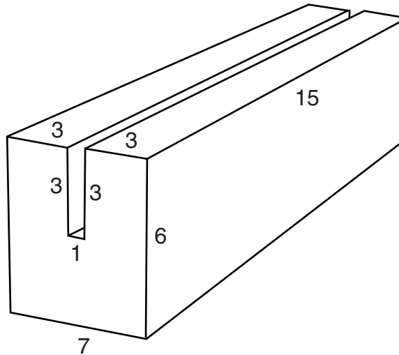
Figure 12–79 Edge seeds for the packaging mesh.
