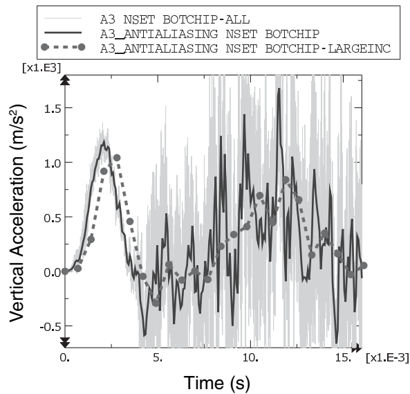
Figure 12–87 Filtered acceleration with different output sampling rates.
