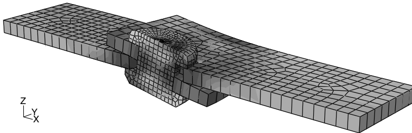
Figure 12–49 Mises stress.
