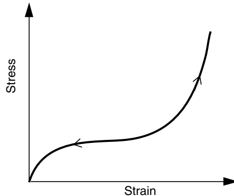
Figure 10–46 Typical stress-strain curve for rubber.
