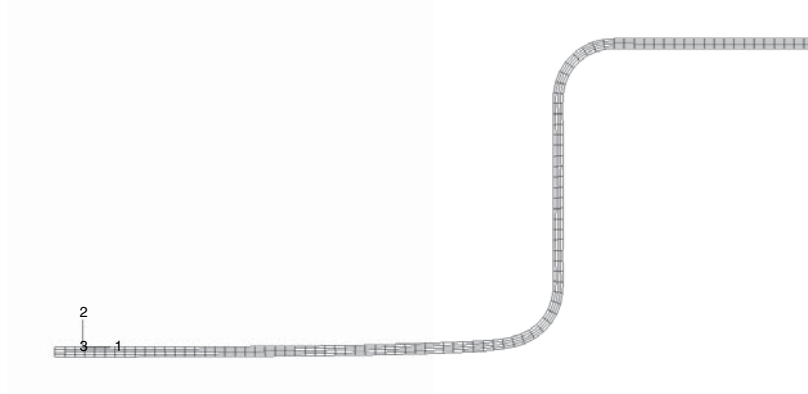
Figure 12–25 Deformed shape of blank at the end of Step 2.
