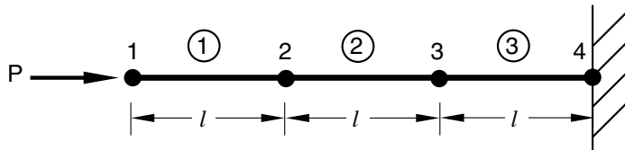
Figure 1–7 Initial configuration of a rod with a concentrated load, P , at the free end.
