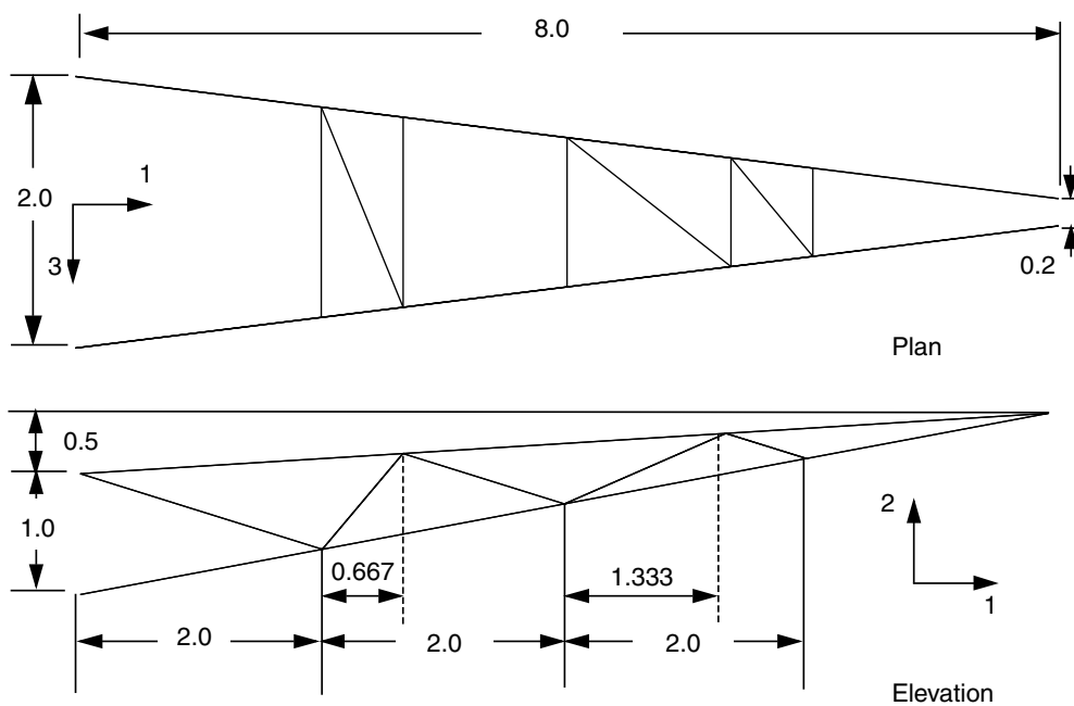
Figure 6-11 Dimensions (in m) of the cargo crane.
