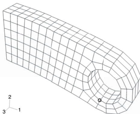
Figure 4–40 Selected node at the bottom of the hole.
